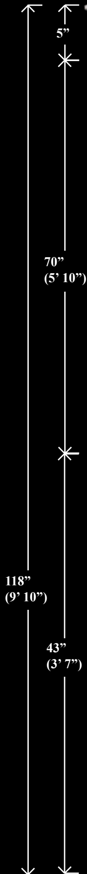
BASE-135 4-3/8" Width 42-3/4" Tall 2-1/2" Depth
