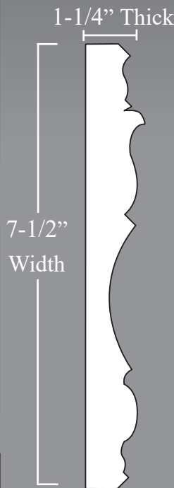
FRZ-440B-2 Bottom Repeat: 7-1/2" Bottom Insert: MLD-135C
