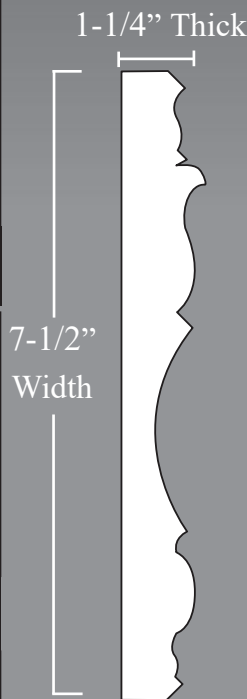
FRZ-440D-2 Bottom Repeat: 7-1/2" Bottom Insert: MLD-135C
