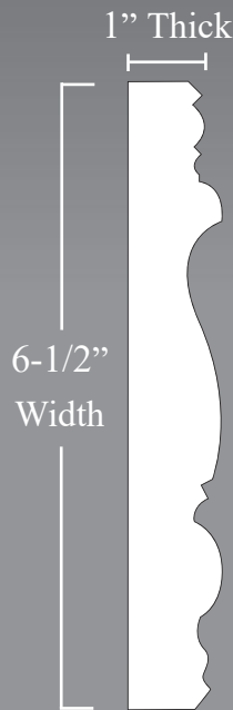
FRZ-430C-2 Bottom Repeat: 7-1/2" Bottom Insert: MLD-135C
