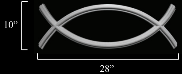
FRZ-162B 28" x 10" x 1/2"
