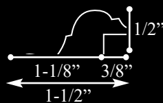
MLD-174 Profile
