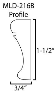
Connection Moulding
